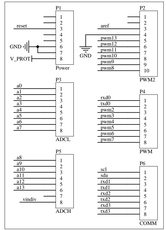
Arduino Mega 2560 R3 connectors
